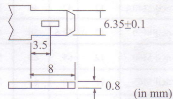
F3(Fasten Tab No.250A)
